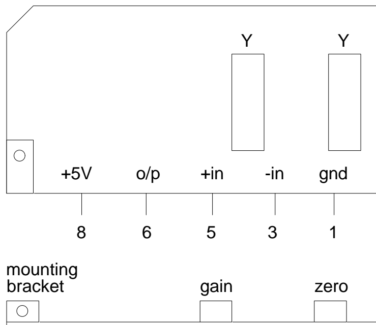
Isolated Input Amplifier (Model 6107A)
