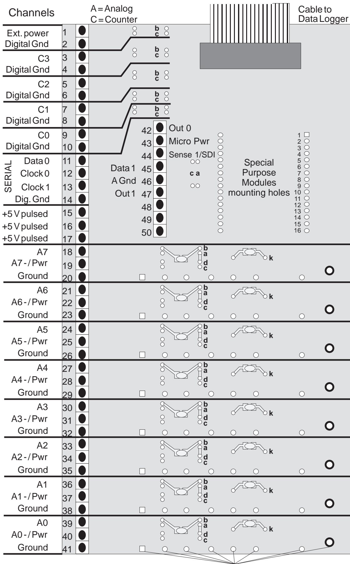
Amplifier module mounting holes Model 6103D Field Termination Strip (front side)
